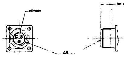
THIS CONNECTOR ACCOMMODATES ANY CONNECTOR THAT MATES WITH MS 3402-108L-3P AERODYNAMIC BRAKE POSITION TRANSDUCER SCHEMATIC OF PIN DESIGNATION
